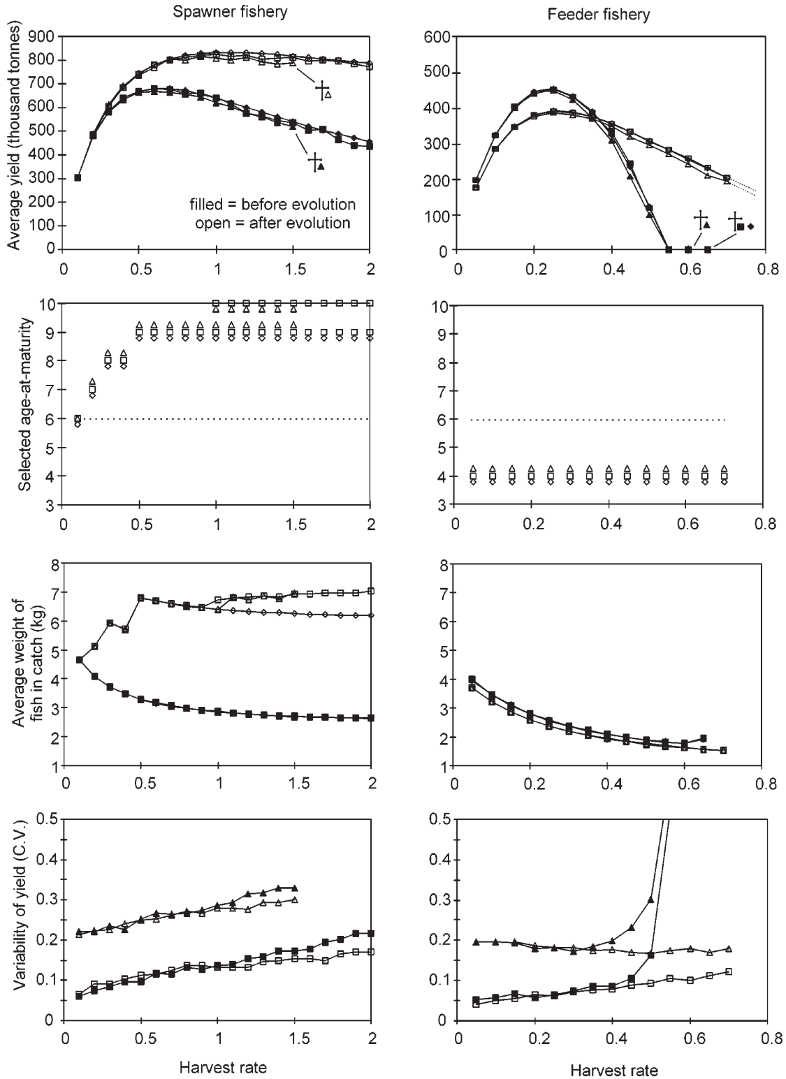
Fig. 2. Sustainable yield in the spawner fishery (selective harvesting of only mature individuals after spawning) and in the feeder fishery (unselective harvesting of immature and mature fish) for different constant harvest rate strategies. Filled symbols indicate the situation for the original life history maturing at age 6. Open symbols are for life histories selected by given harvest rates. Diamonds, deterministic model; squares, stochastic model with noise in newborn survival; triangles, stochastic model with noise in newborn survival and inaccurate estimate of stock size. Crosses indicate that greedier harvest strategies result in extinction. Harvesting at the spawner fishery selects for delayed maturation and results in increased sustainable yield and average weight of caught fish and decreased variation in annual catch. Harvesting at the feeding grounds selects for earlier maturation and results in decreased sustainable yield and a minor decrease in fish weight.
