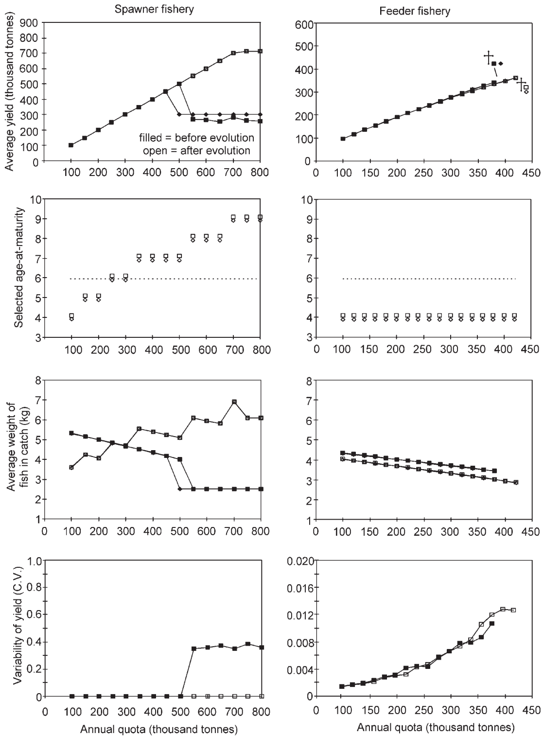
Fig. 4. Performance of spawner and feeder fisheries managed with a fixed-quota strategy. See Fig. 2 for further explanation and Figs. 2 and 3 for comparison.
