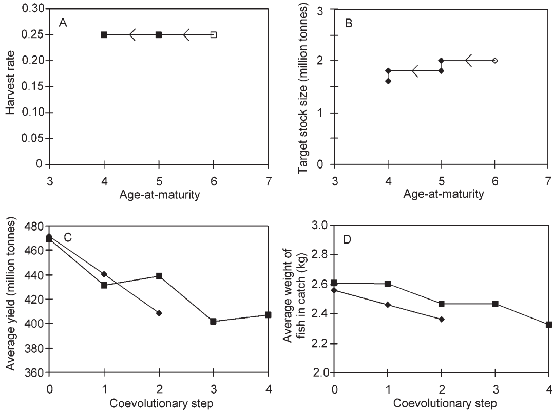
Fig. 6. Coevolutionary dynamics of a fish stock and the manager adopting (A) a constant harvest rate strategy (B) or a constant stock size strategy in a feeder fishery (unselective harvesting of immature and mature fish) and change in (C) average yields and (D) fish weight. The final harvest strategy is an ESOHS. See Fig. 5 for description of the coevolutionary process.
