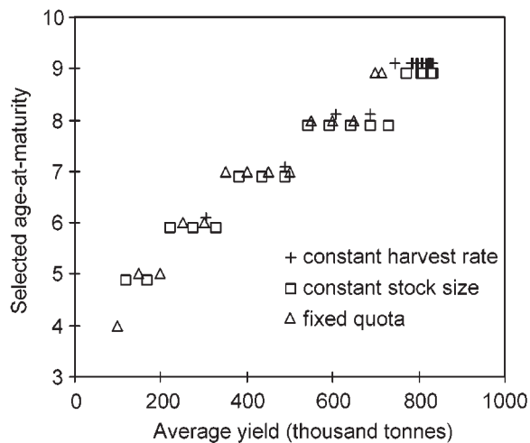
Fig. 7. Comparison of the evolutionary consequences of different harvest strategies in the deterministic model.
