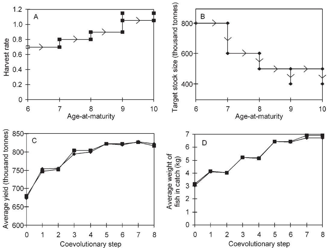
Fig. 5. Coevolutionary dynamics of a fish stock and the manager adopting (A) a constant harvest rate strategy or (B) a constant stock size strategy in a spawner fishery (selective harvesting of mature fish). The model assumes stochasticity in newborn survival. The manager first chooses an optimal strategy (i.e., the strategy that results in MSY) for the original fish life history (open symbols). The fish stock then evolves in response to the harvesting; it is assumed that age-at-maturity can change only for 1 year at a time. The coevolutionary dynamics reach a state in which it is advantageous for neither the fish nor the manager to change the strategy; at this state, the fish stock is polymorphic. Further, the strategy that the manager adopts is an ESOHS (see text for explanation of the term). In the course of coevolutionary change, (C) average yield and (D) fish weight increase. Diamonds, constant harvest rate strategy; squares, constant stock size strategy.
