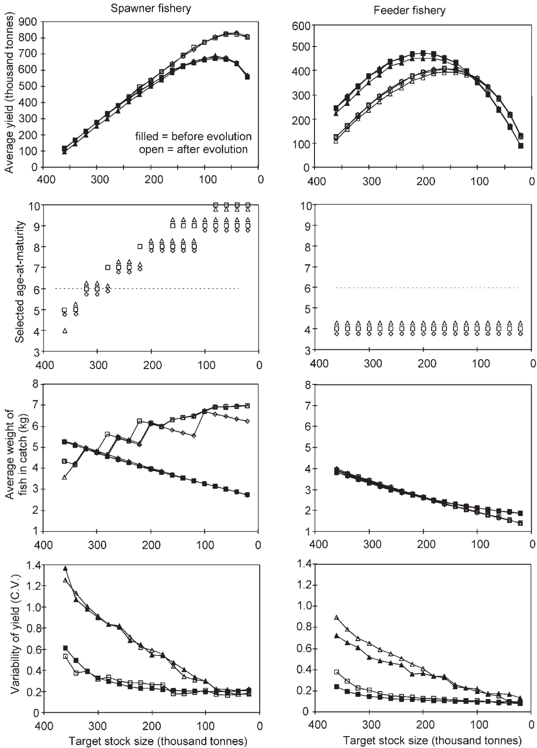
Fig. 3. Performance and evolutionary consequences of harvesting with a constant stock size strategy, i.e., an excess biomass above a certain threshold is harvested. See Fig. 2 for further explanation and for comparison.
