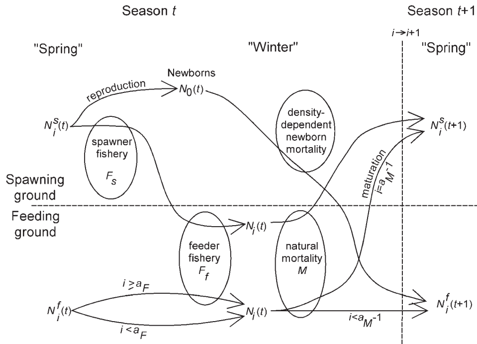
Fig. 1. Schematic representation of the age- and stage-structured population dynamics model for the Northeast Arctic cod. N_i denotes the size of age-class i at the feeding grounds during the late season after fishing but before natural mortality. Superscripts "s" and "f" refer to the abundances at the spawning and feeding grounds, respectively, during the early season at the time of reproduction. Mature fish (age \geq a_M ) are harvested at the spawning grounds at rate F_s . Both mature and immature fish at least a_F years old are harvested at the feeding grounds at rate F_f .
